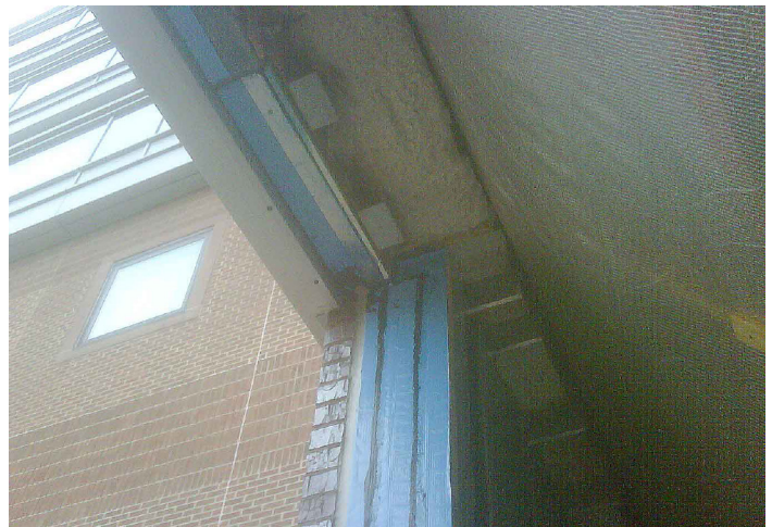
Example 2D: Jamb to head intersection
