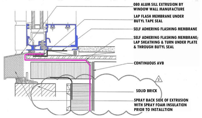
Example 2: Sill detail showing inappropriate location of the primary seal of the glazing system.
