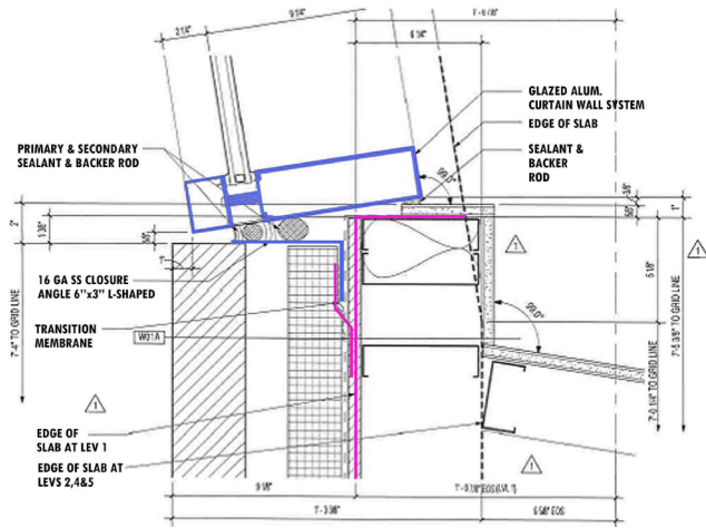
Example 1A: Shop drawing section detail at splayed jamb
