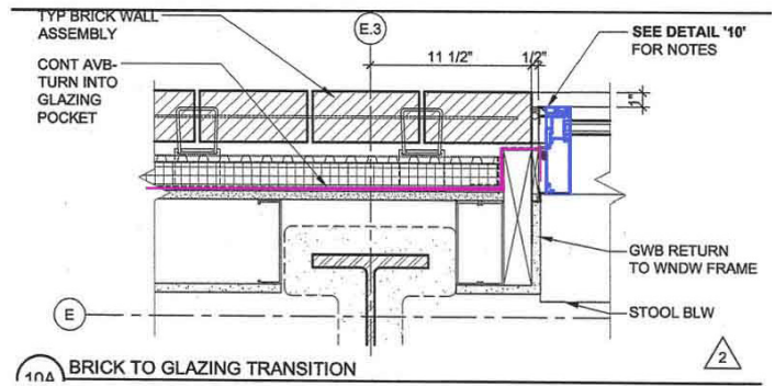
Example 2A: Jamb detail at brick to glazing transition
