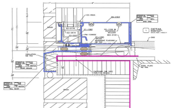
Example 2B: Shop drawing sill detail
