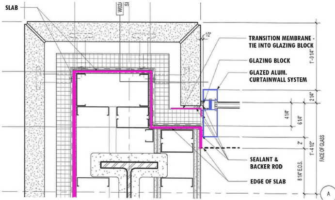
Example 1: Section detail at jamb showing inappropriate location of the primary seal of the glazing system.
