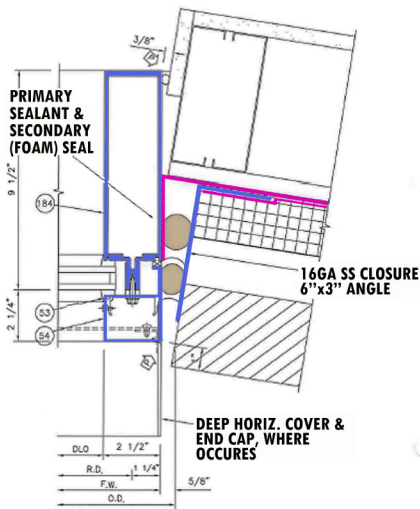
Example 1B: Revised shop drawing section detail at splayed jamb
